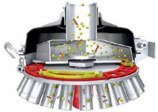
The DosiMat distributor head ensures that slurry is distributed homogeneously.
